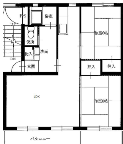
2LDK-A(2-11)
